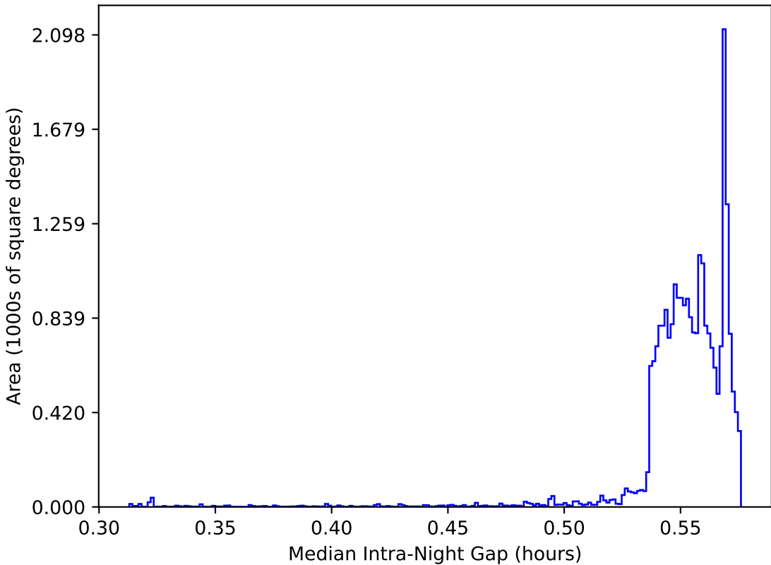
reweight_plane_v3.3_10yrs All sky: Median Intra-Night Gap
