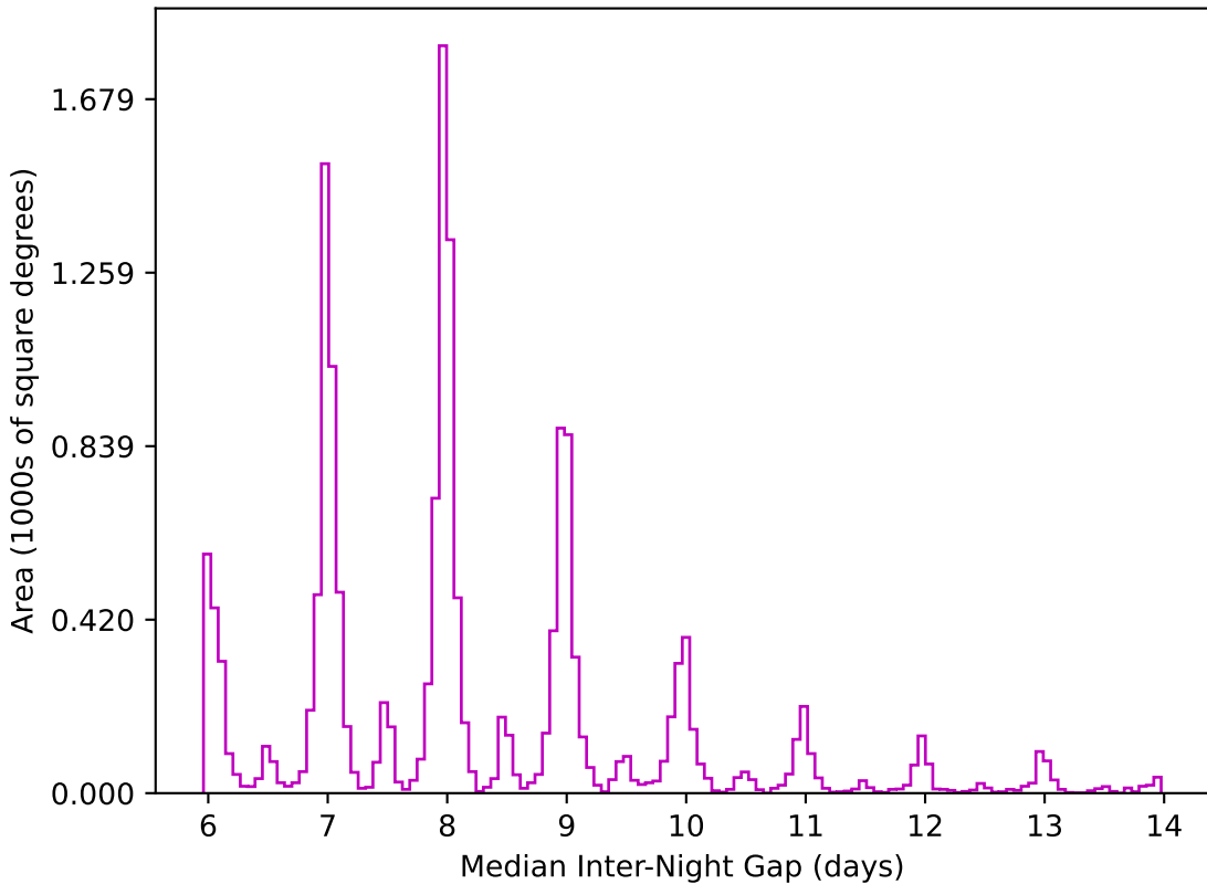
reweight_plane_v3.3_10yrs WFD z band: Median Inter-Night Gap
