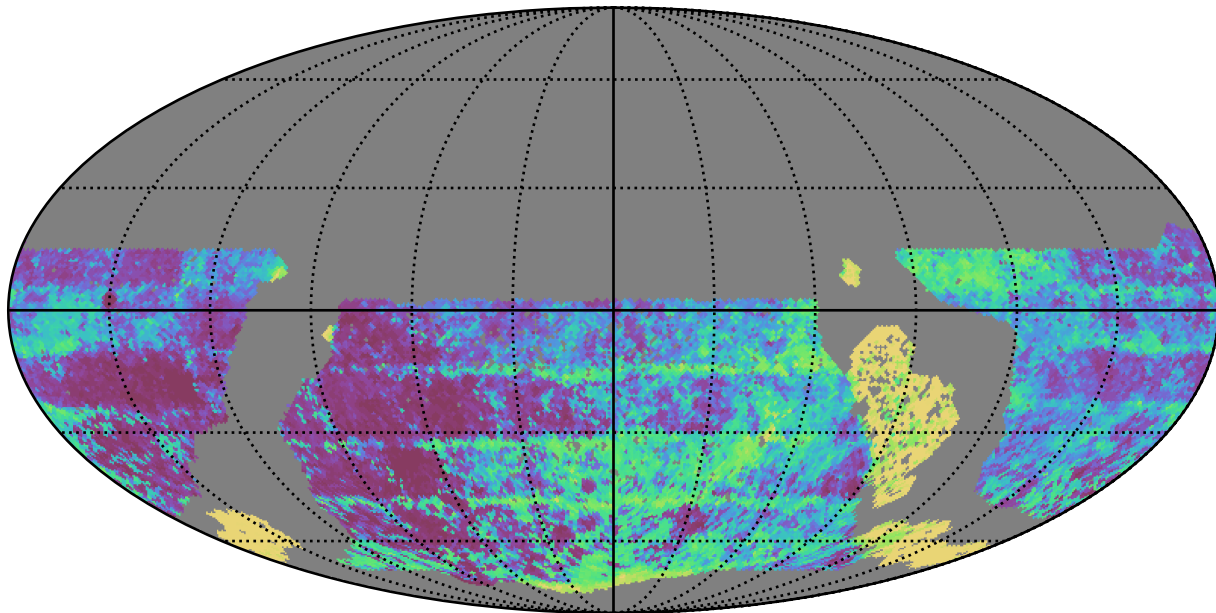
reweight_plane_v3.3_10yrs WFD y band: Median Inter-Night Gap
