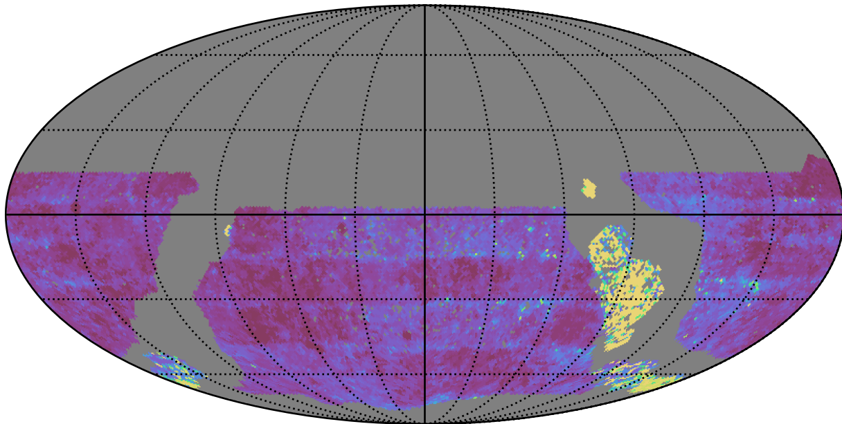
reweight_plane_v3.3_10yrs WFD u band: Median Inter-Night Gap
