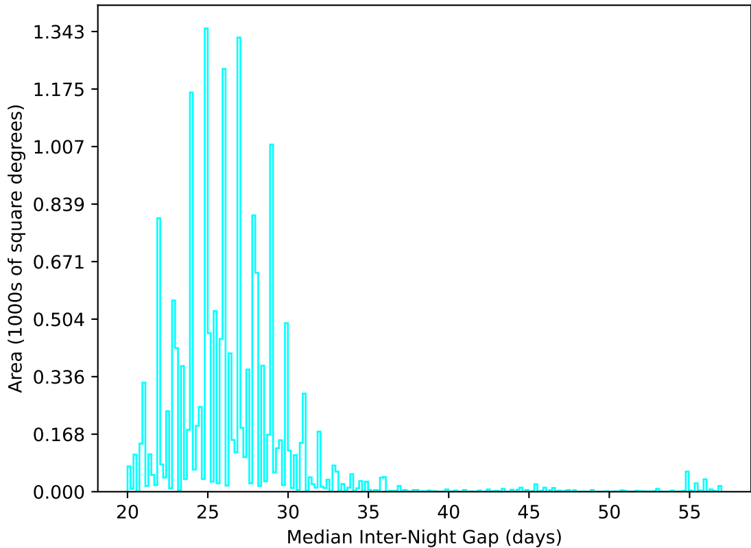
reweight_plane_v3.3_10yrs WFD u band: Median Inter-Night Gap
