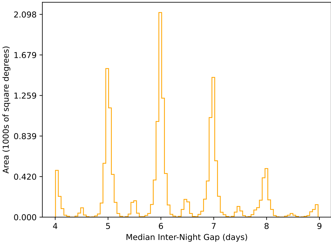
reweight_plane_v3.3_10yrs WFD r band: Median Inter-Night Gap
