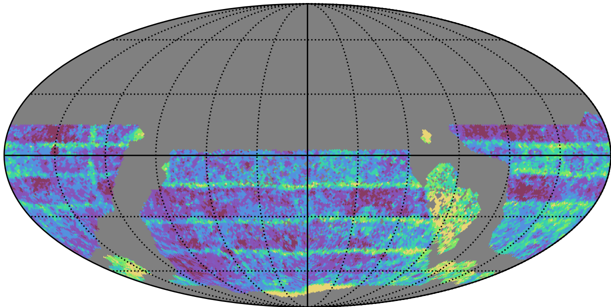
reweight_plane_v3.3_10yrs WFD i band: Median Inter-Night Gap
