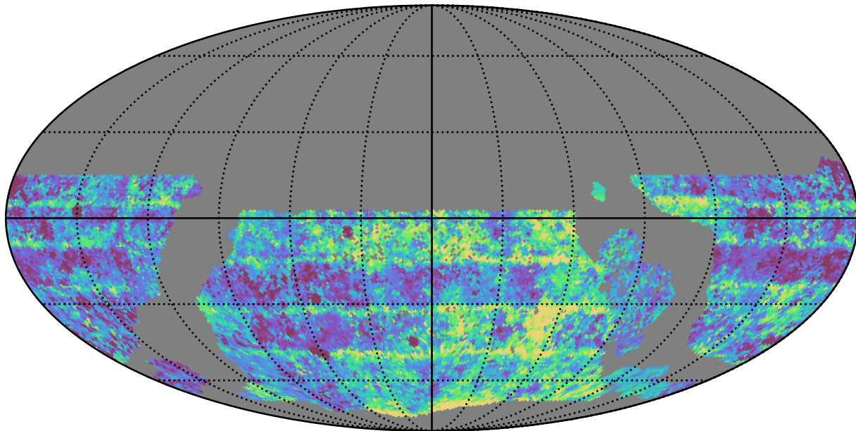
reweight_plane_v3.3_10yrs WFD g band: Median Inter-Night Gap
