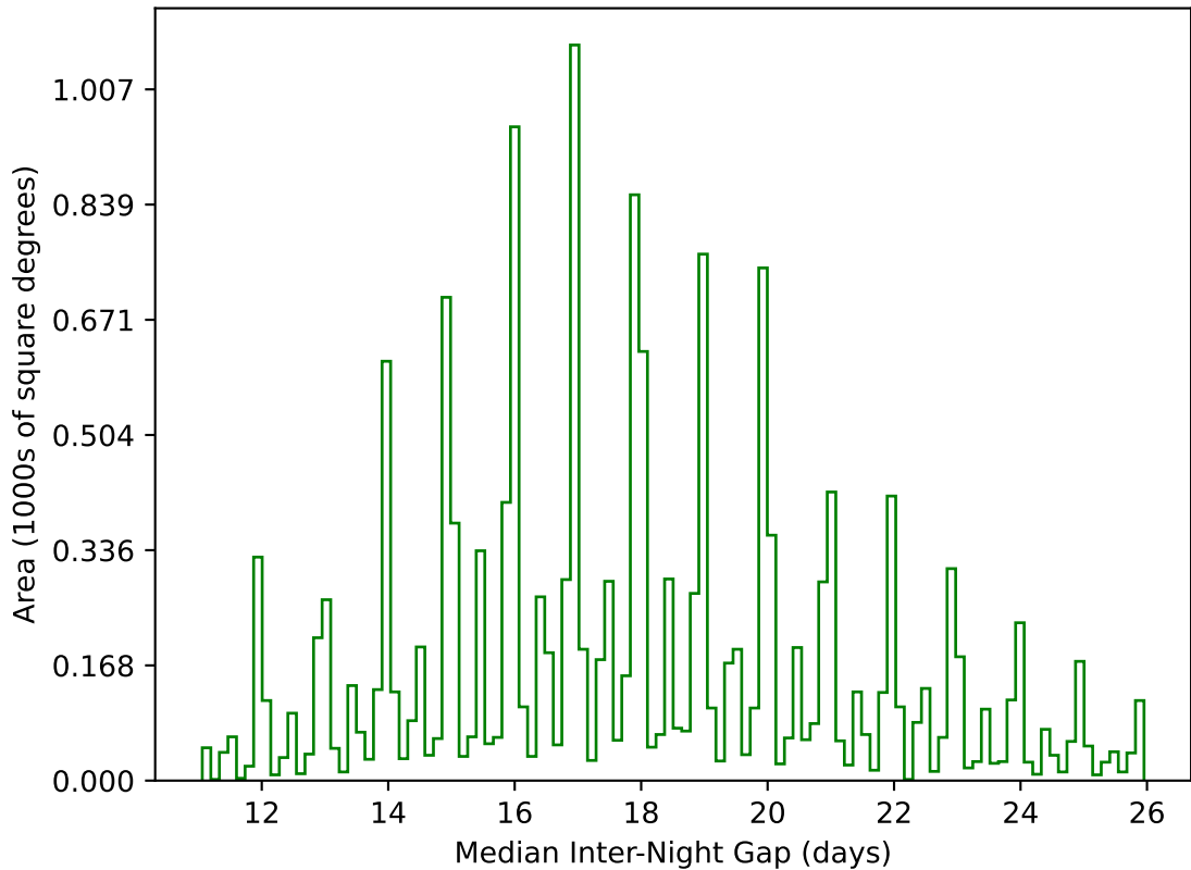
reweight_plane_v3.3_10yrs WFD g band: Median Inter-Night Gap
