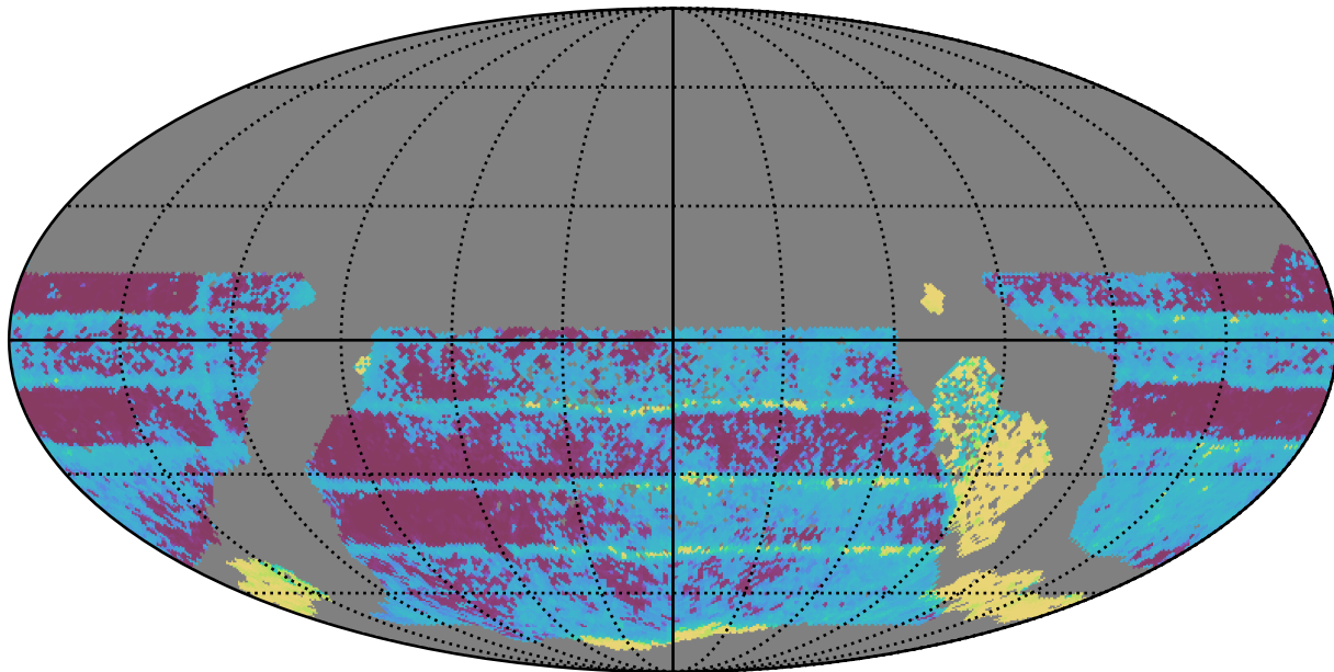
reweight_plane_v3.3_10yrs WFD all bands: Median Inter-Night Gap
