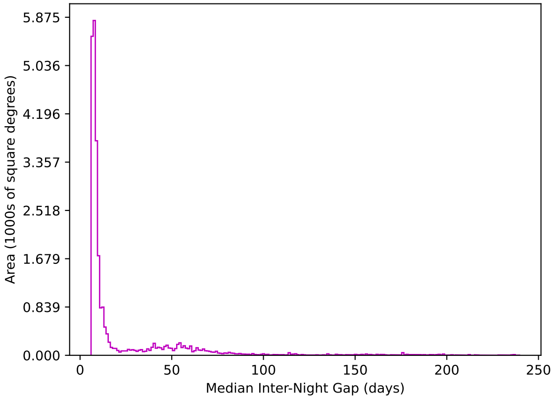
reweight_plane_v3.3_10yrs All sky z band: Median Inter-Night Gap
