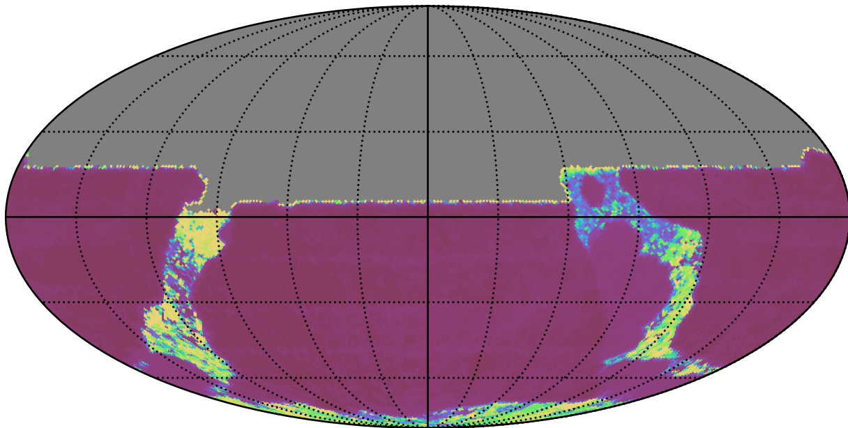
reweight_plane_v3.3_10yrs All sky y band: Median Inter-Night Gap
