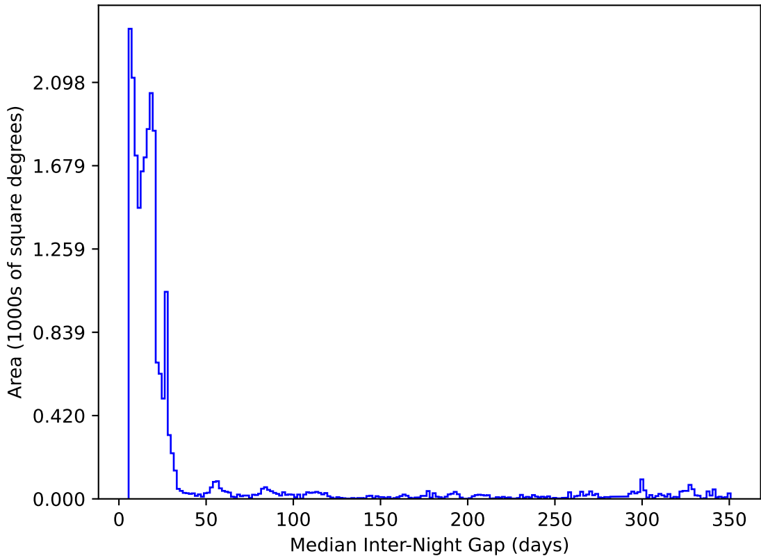
reweight_plane_v3.3_10yrs All sky y band: Median Inter-Night Gap
