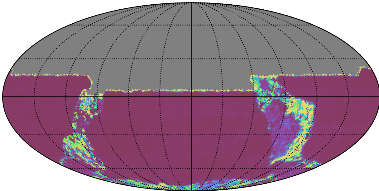
reweight_plane_v3.3_10yrs All sky u band: Median Inter-Night Gap
