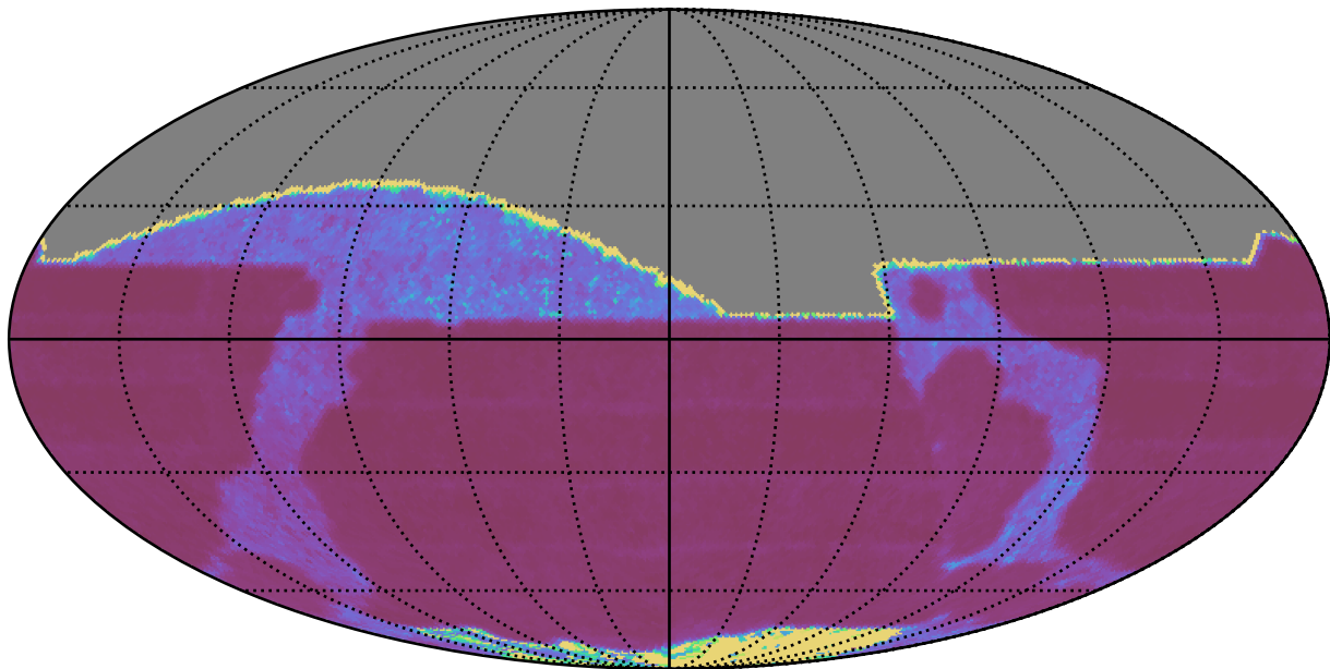
reweight_plane_v3.3_10yrs All sky r band: Median Inter-Night Gap
