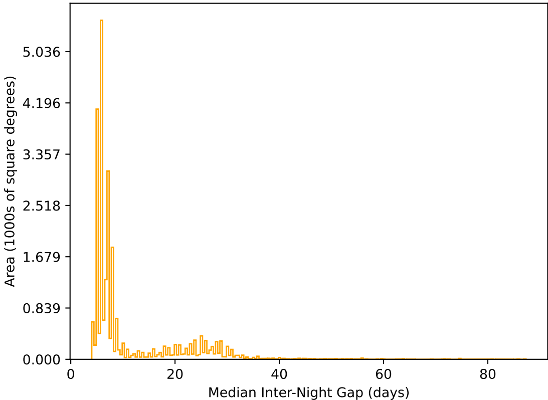
reweight_plane_v3.3_10yrs All sky r band: Median Inter-Night Gap
