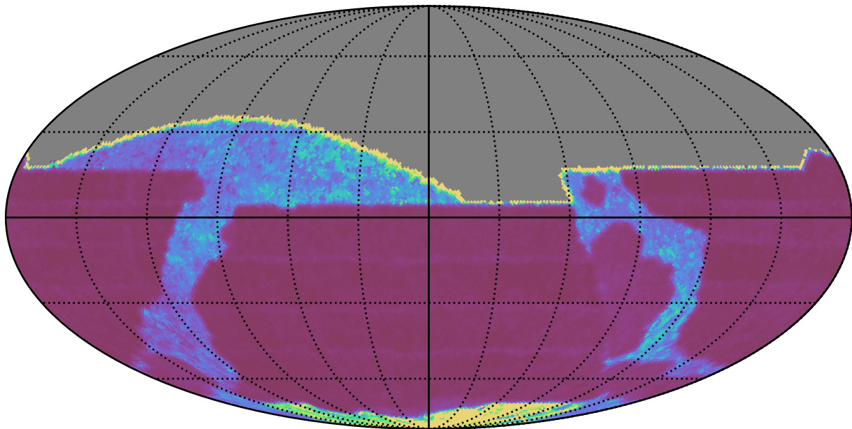
reweight_plane_v3.3_10yrs All sky i band: Median Inter-Night Gap
