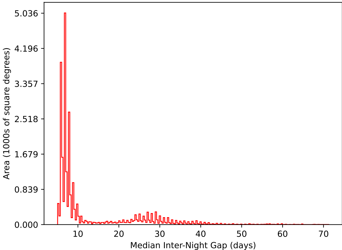
reweight_plane_v3.3_10yrs All sky i band: Median Inter-Night Gap
