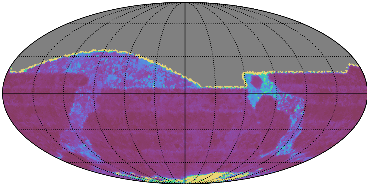
reweight_plane_v3.3_10yrs All sky g band: Median Inter-Night Gap
