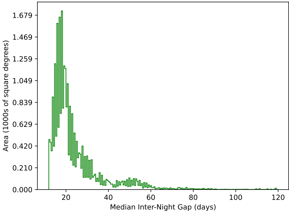
reweight_plane_v3.3_10yrs All sky g band: Median Inter-Night Gap
