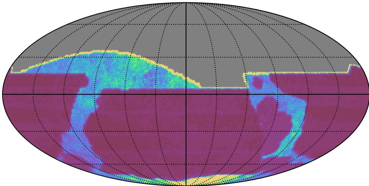
reweight_plane_v3.3_10yrs All sky all bands: Median Inter-Night Gap
