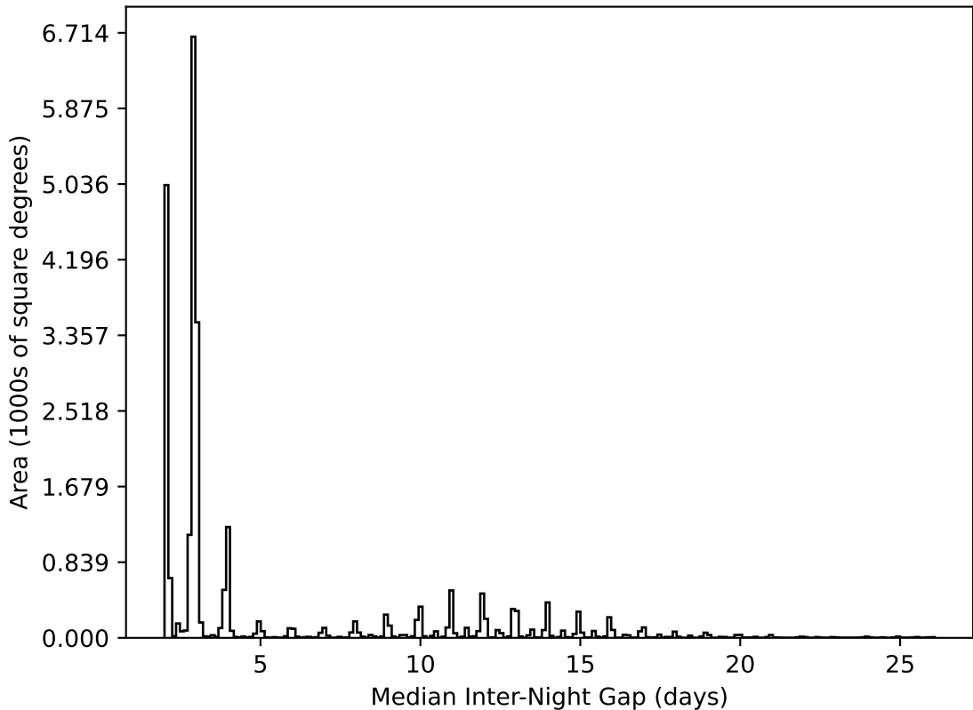
reweight_plane_v3.3_10yrs All sky all bands: Median Inter-Night Gap
