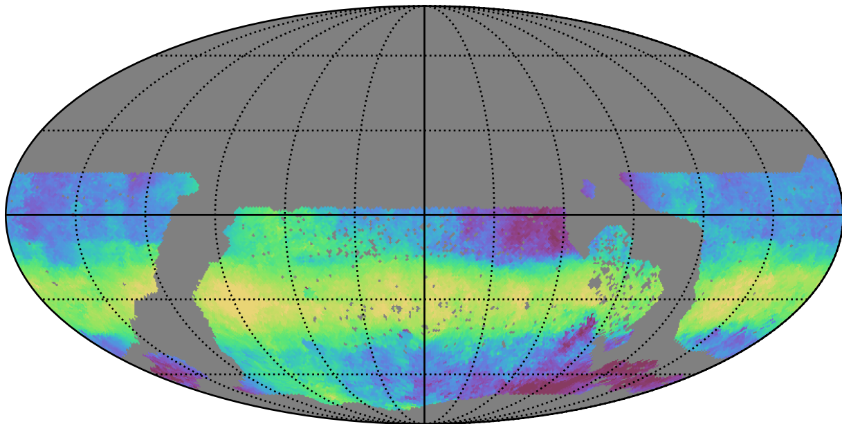
reweight_plane_v3.3_10yrs WFD z band: Median HA
