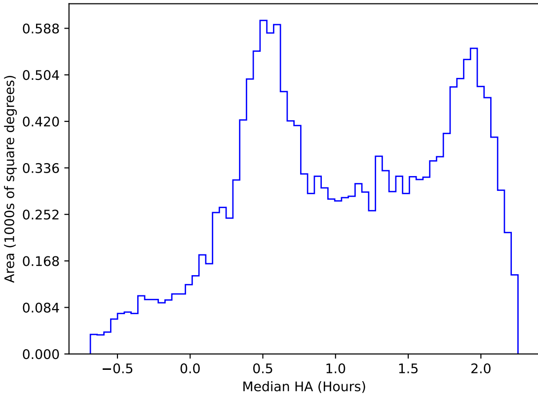
reweight_plane_v3.3_10yrs WFD z band: Median HA
