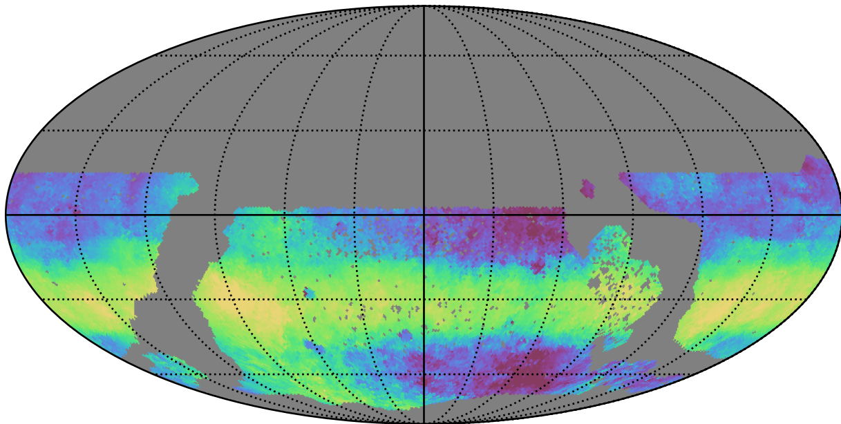
reweight_plane_v3.3_10yrs WFD y band: Median HA
