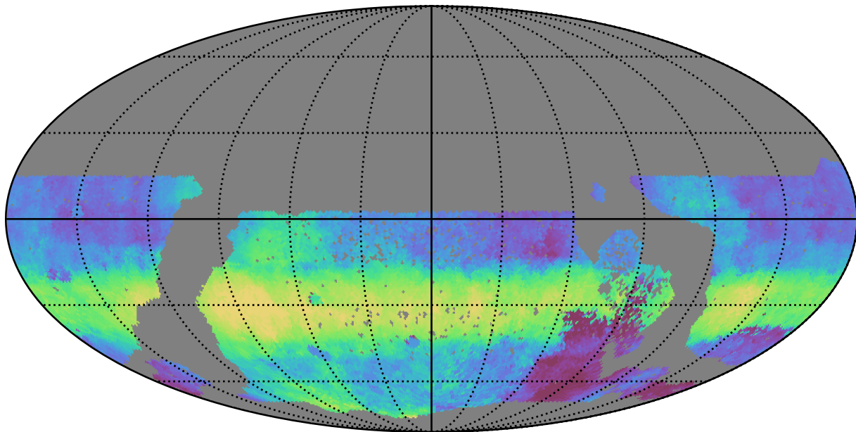
reweight_plane_v3.3_10yrs WFD r band: Median HA
