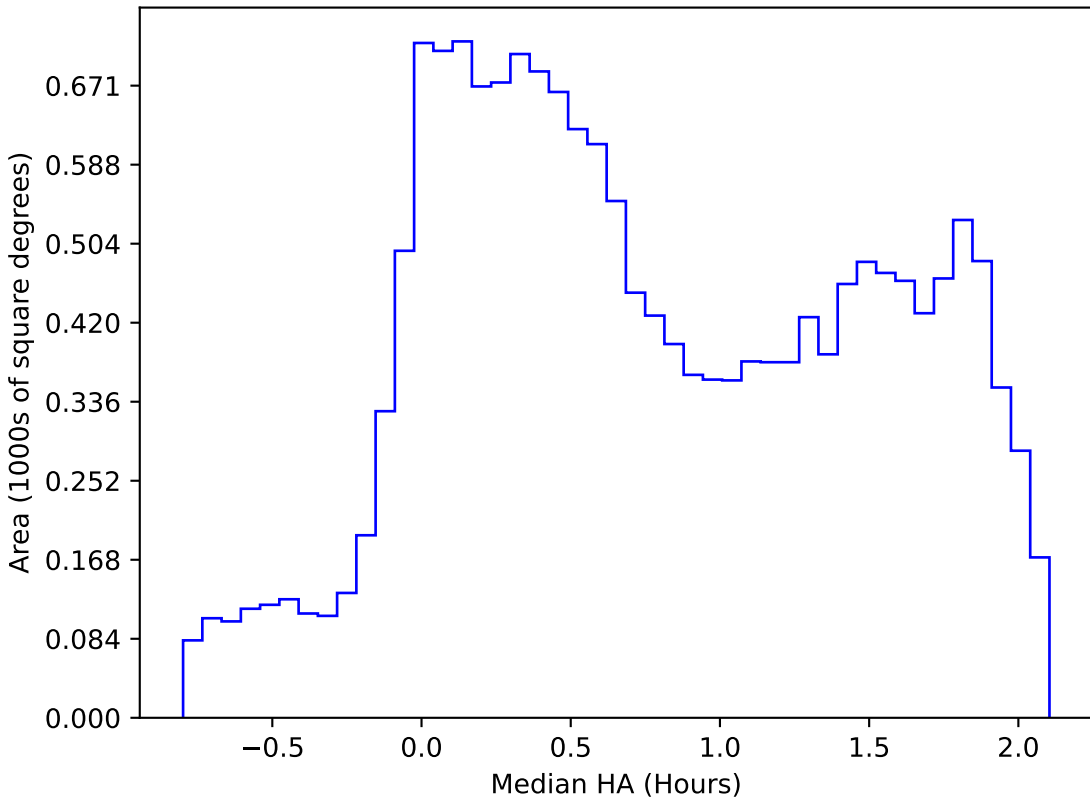
reweight_plane_v3.3_10yrs WFD r band: Median HA
