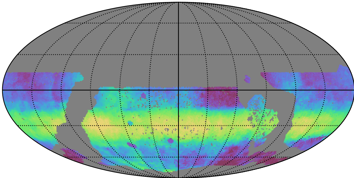
reweight_plane_v3.3_10yrs WFD i band: Median HA
