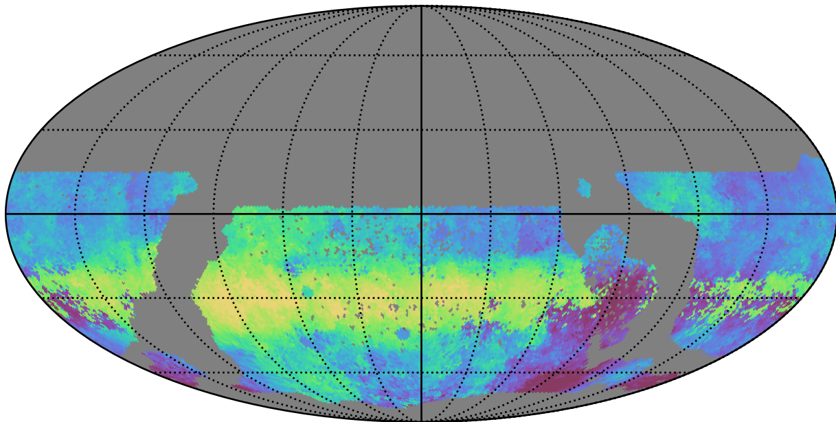
reweight_plane_v3.3_10yrs WFD g band: Median HA
