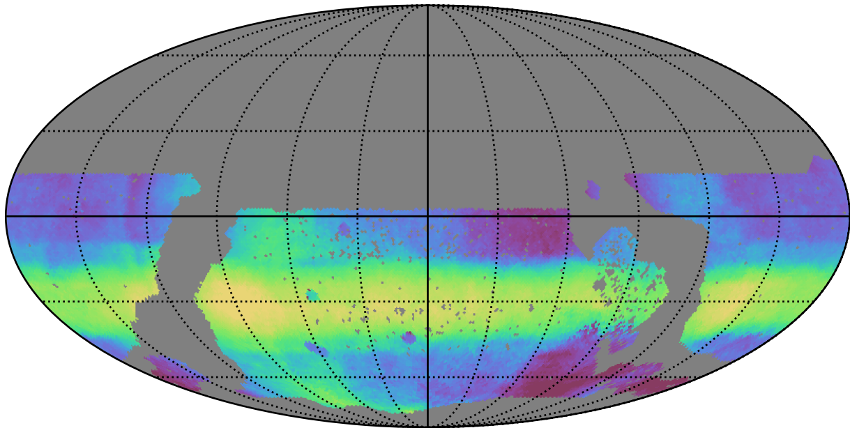
reweight_plane_v3.3_10yrs WFD all bands: Median HA
