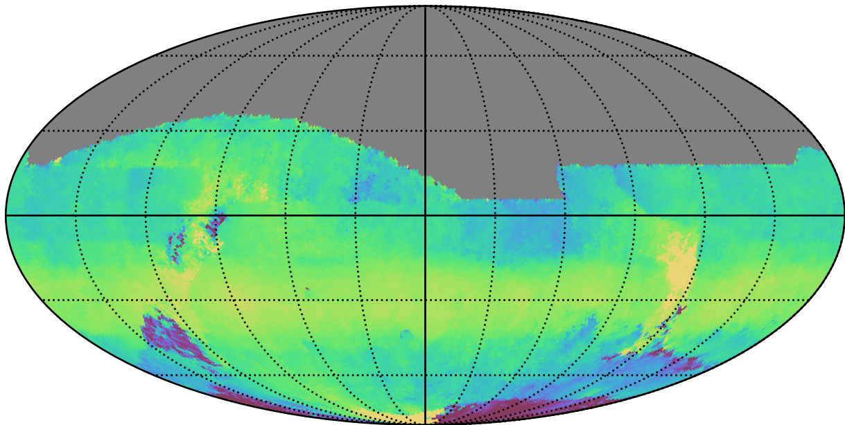
reweight_plane_v3.3_10yrs All sky z band: Median HA
