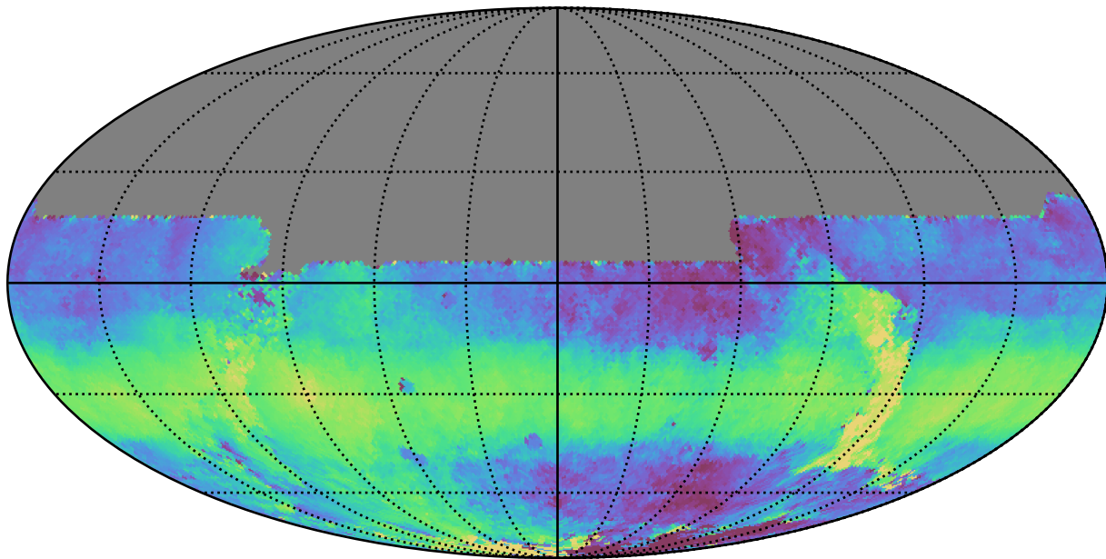
reweight_plane_v3.3_10yrs All sky y band: Median HA
