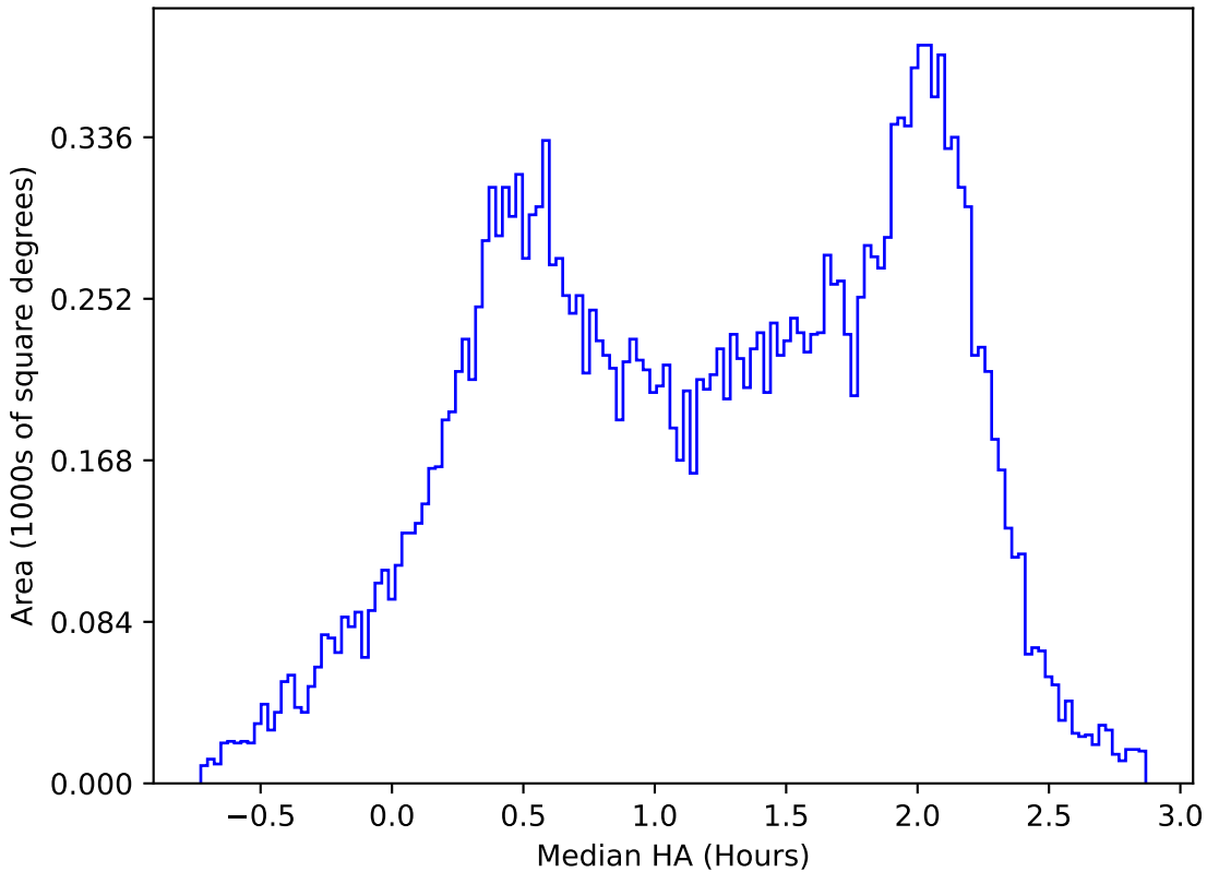
reweight_plane_v3.3_10yrs All sky y band: Median HA
