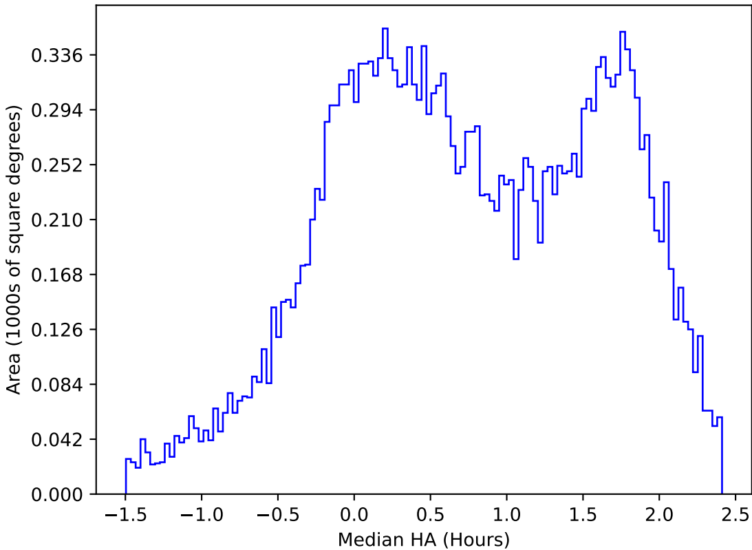
reweight_plane_v3.3_10yrs All sky u band: Median HA
