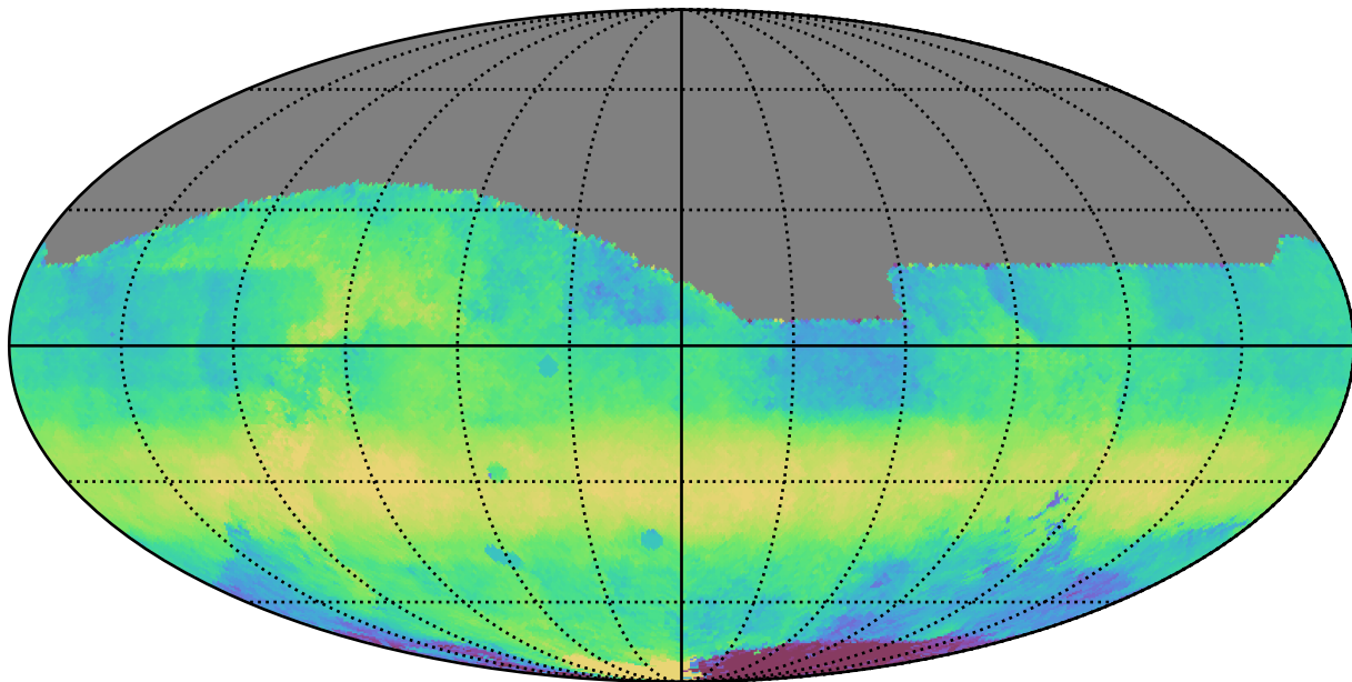
reweight_plane_v3.3_10yrs All sky i band: Median HA
