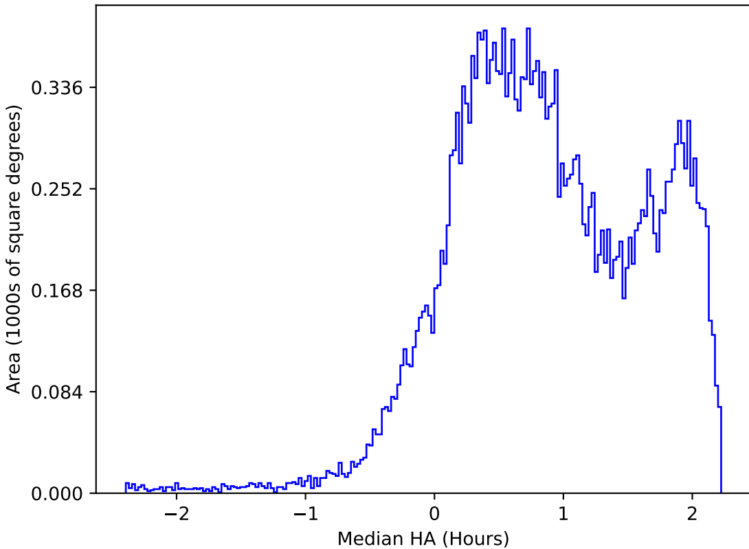
reweight_plane_v3.3_10yrs All sky i band: Median HA
