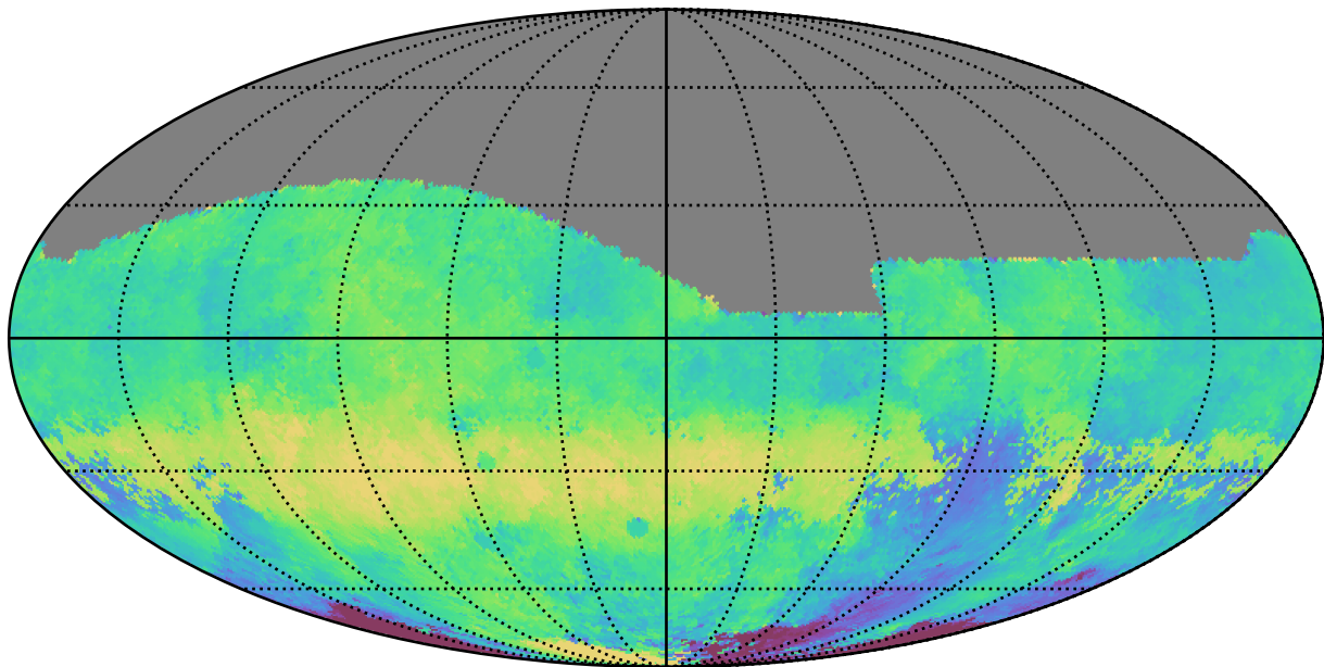
reweight_plane_v3.3_10yrs All sky g band: Median HA
