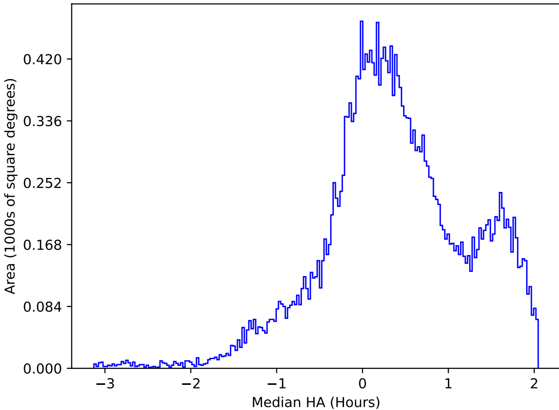
reweight_plane_v3.3_10yrs All sky g band: Median HA
