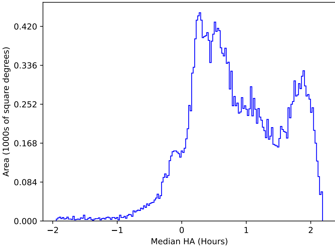
reweight_plane_v3.3_10yrs All sky all bands: Median HA
