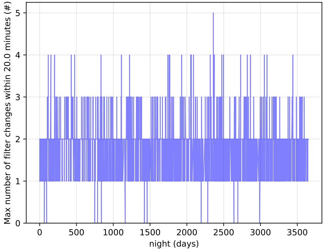
reweight_plane_v3.3_10yrs Per Night: Max number of filter changes within 20.0 minutes
