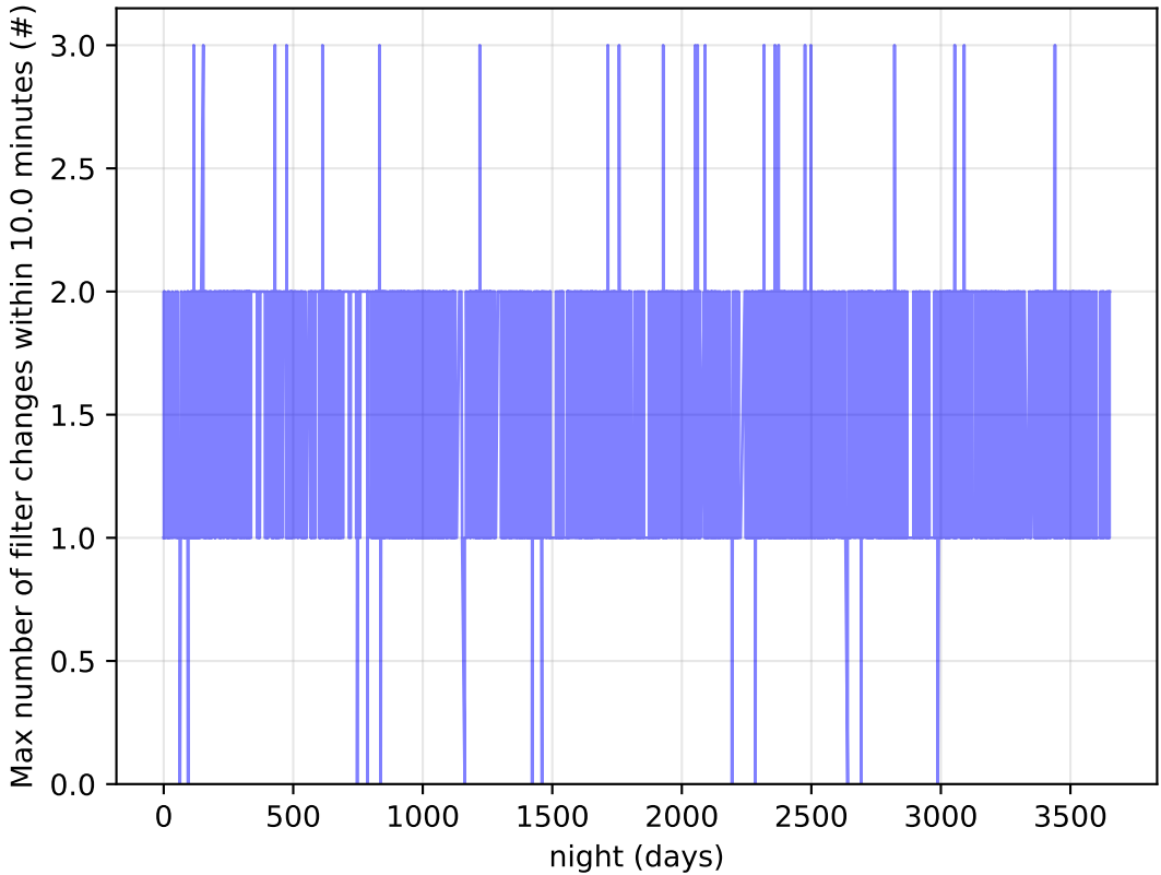
reweight_plane_v3.3_10yrs Per Night: Max number of filter changes within 10.0 minutes
