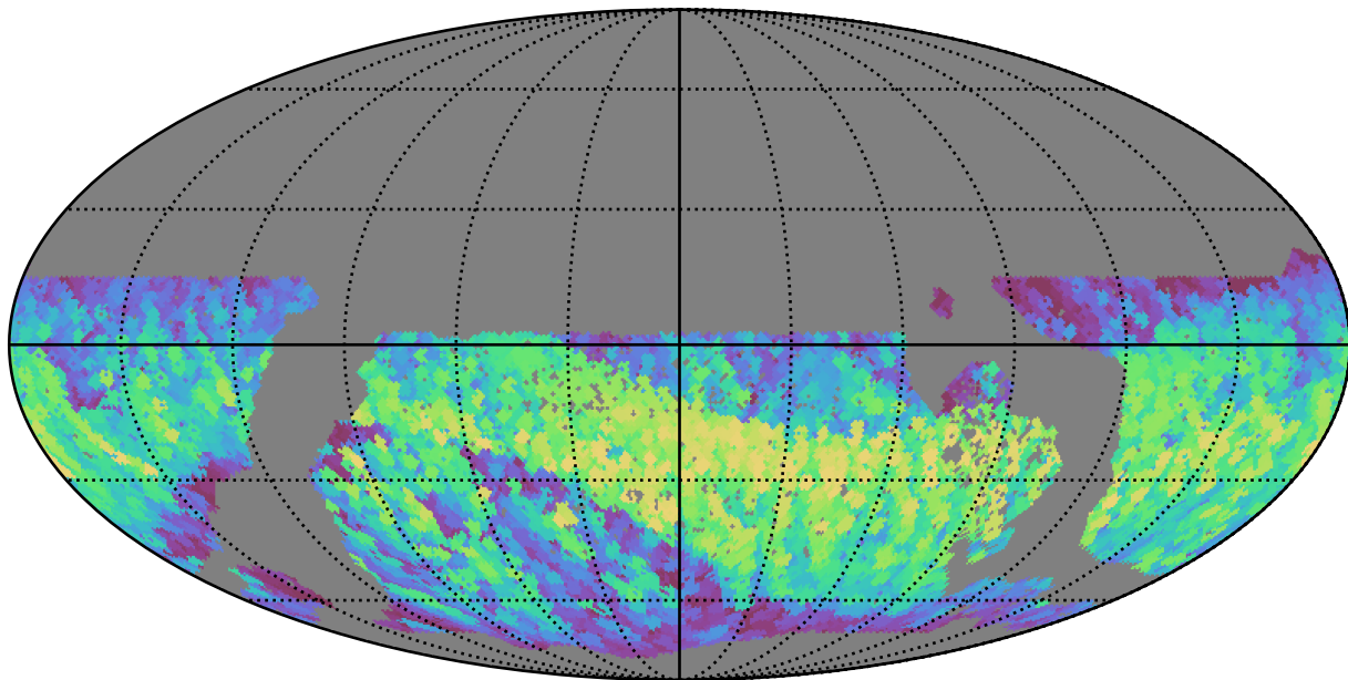
reweight_plane_v3.3_10yrs WFD z band: Max normairmass
