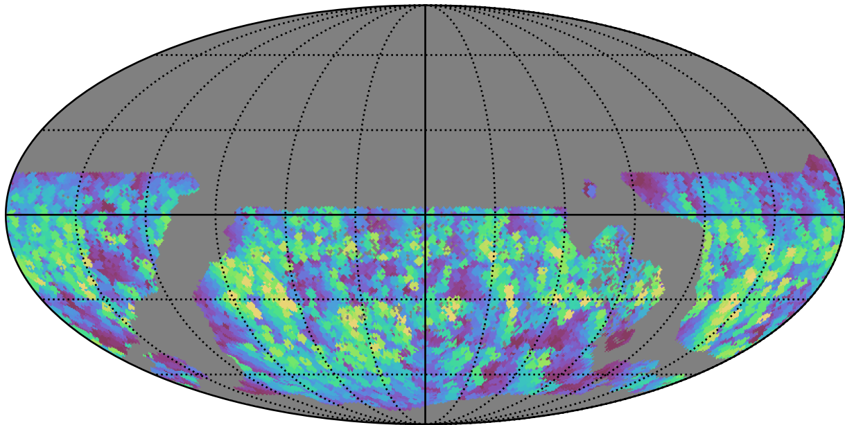
reweight_plane_v3.3_10yrs WFD y band: Max normairmass
