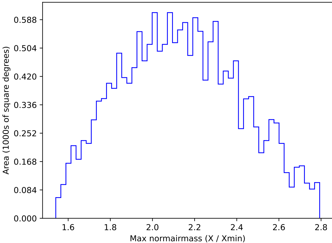
reweight_plane_v3.3_10yrs WFD y band: Max normairmass
