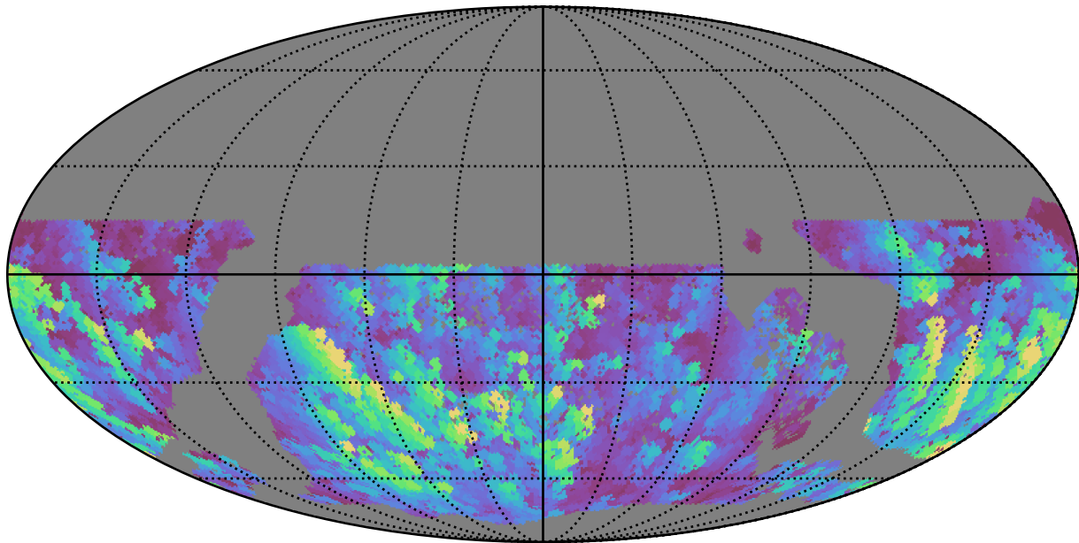
reweight_plane_v3.3_10yrs WFD u band: Max normairmass
