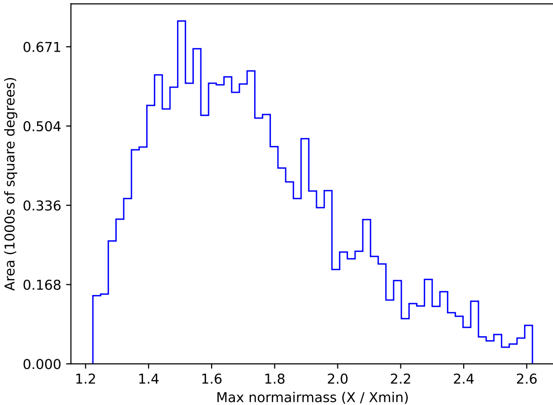
reweight_plane_v3.3_10yrs WFD u band: Max normairmass
