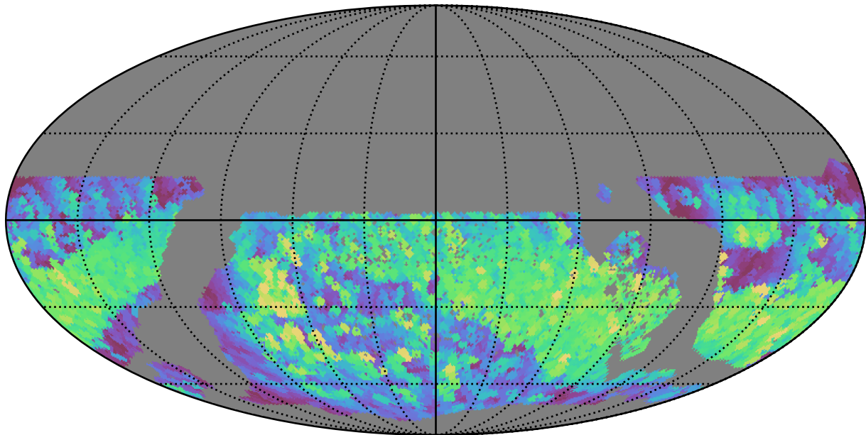
reweight_plane_v3.3_10yrs WFD r band: Max normairmass
