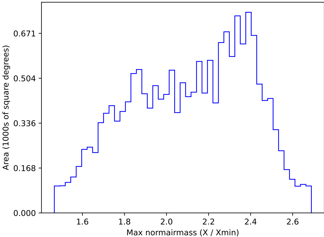
reweight_plane_v3.3_10yrs WFD r band: Max normairmass
