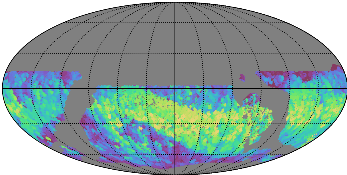
reweight_plane_v3.3_10yrs WFD i band: Max normairmass
