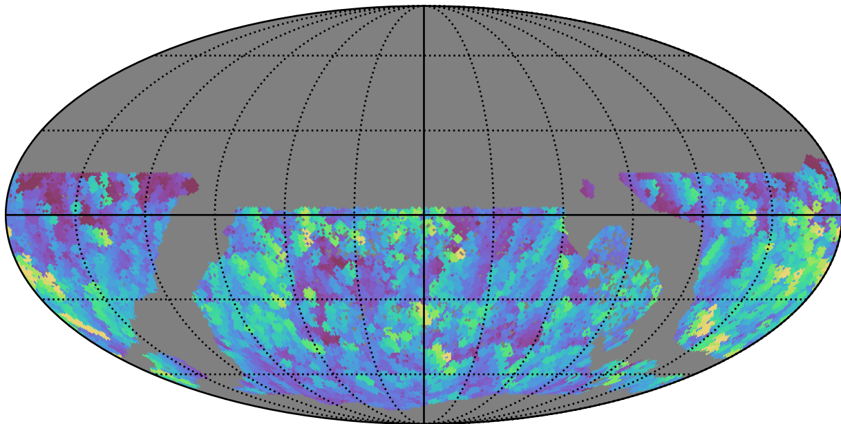
reweight_plane_v3.3_10yrs WFD g band: Max normairmass
